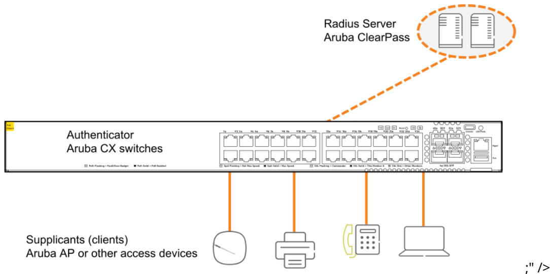
Figure 1 Example of device profile setup along with RADIUS infrastructure
