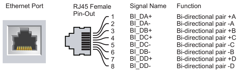
Figure 6 Ethernet Port Pin-Out
