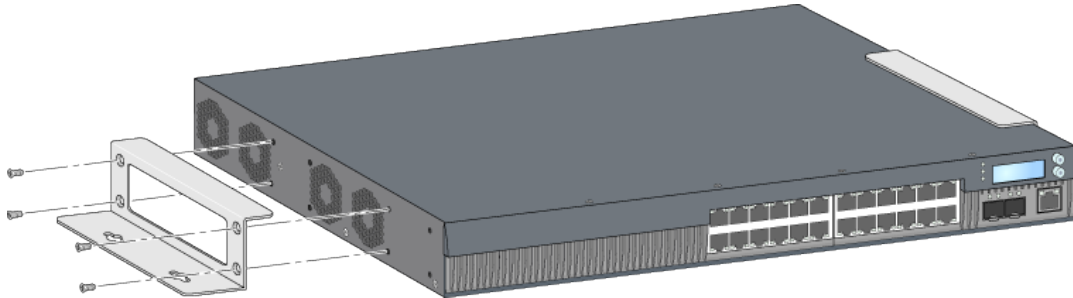
Figure 12 Wall-Mount Brackets
