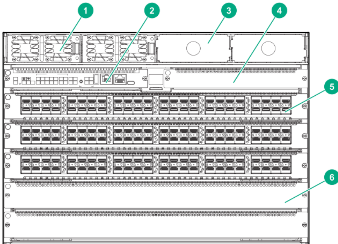
Figure 7 HPE Aruba Networking 6405: front of the switch
