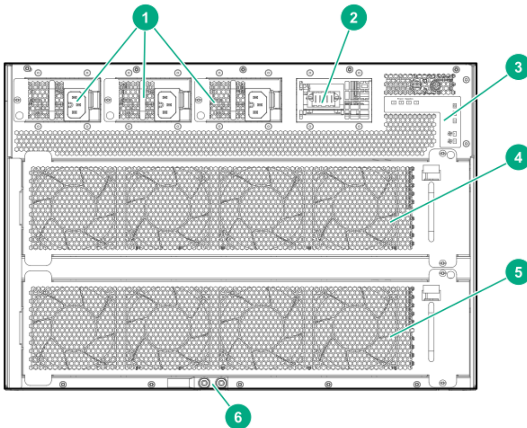
Figure 27 HPE Aruba Networking 6405 rear panel with two fan trays
