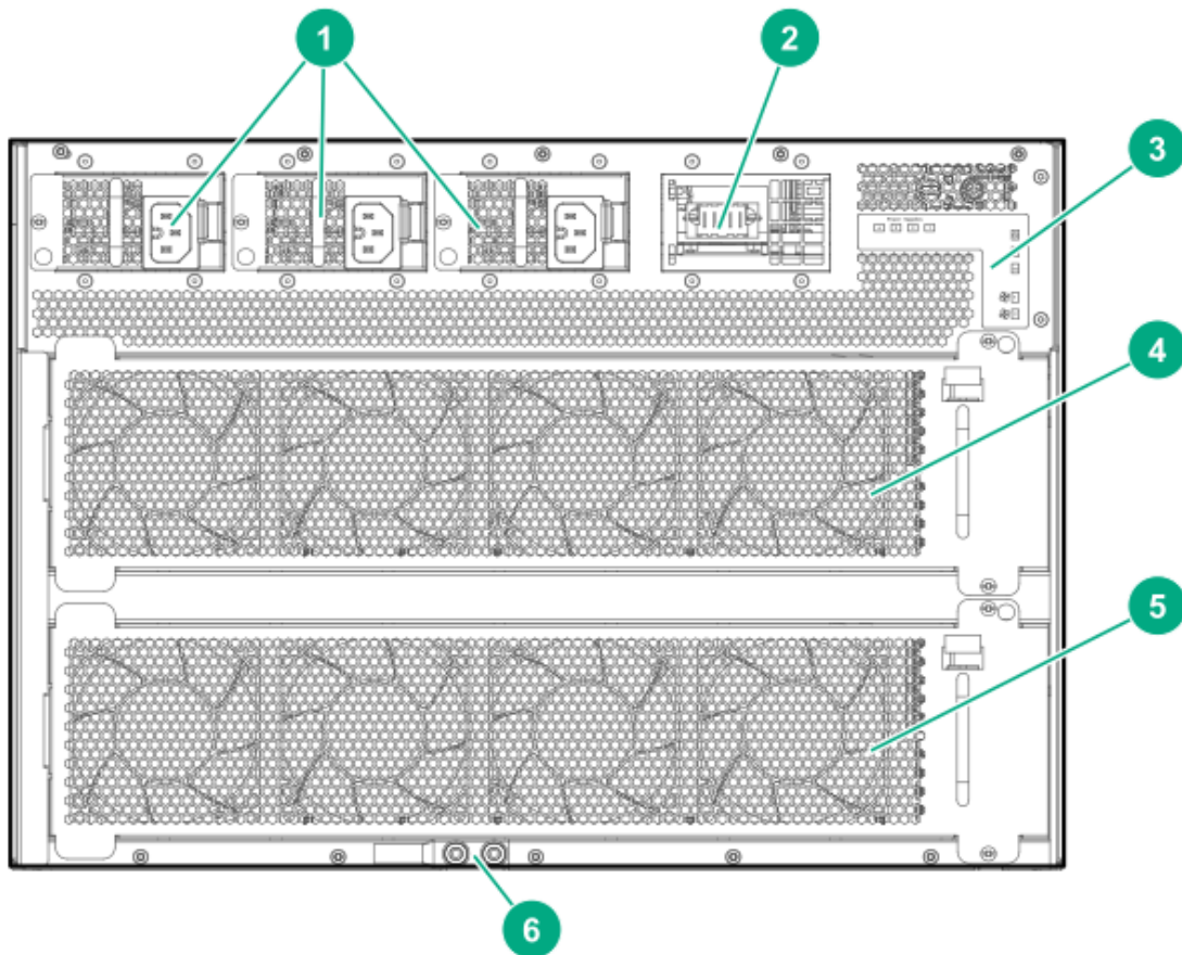
Figure 13 HPE Aruba Networking 6405 rear panel
