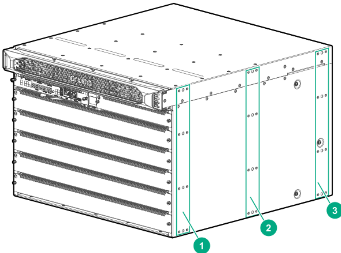
Figure 17 Two-post rack mount options
