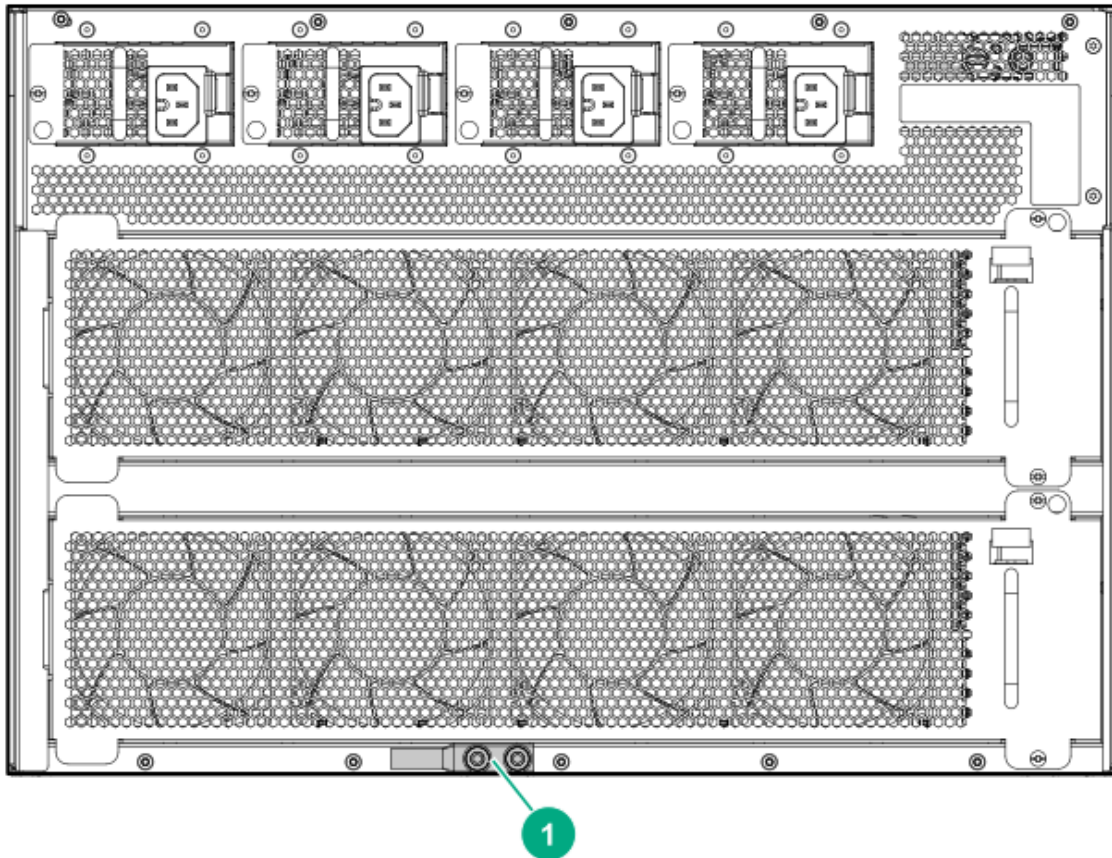
Figure 24 Grounding the chassis
