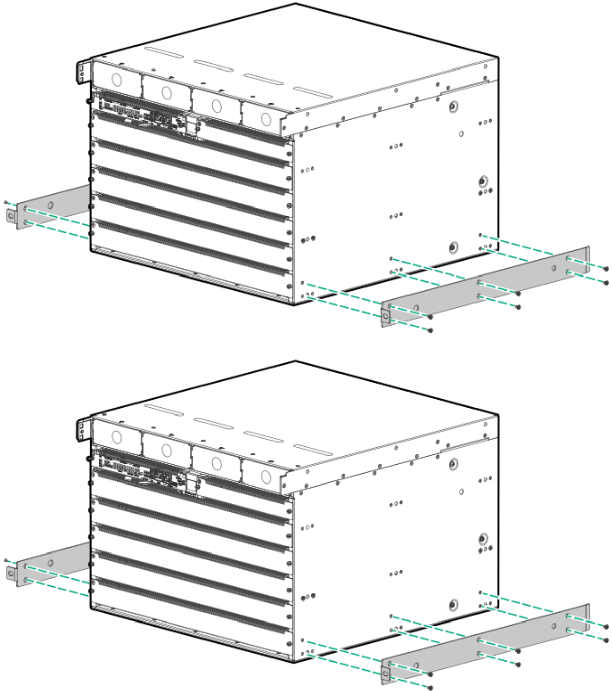
Figure 21 Attaching a rail spacer to each side of the chassis
