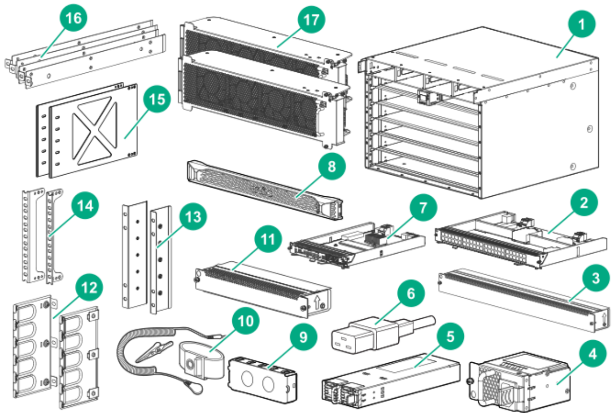
Figure 16 Hardware components
