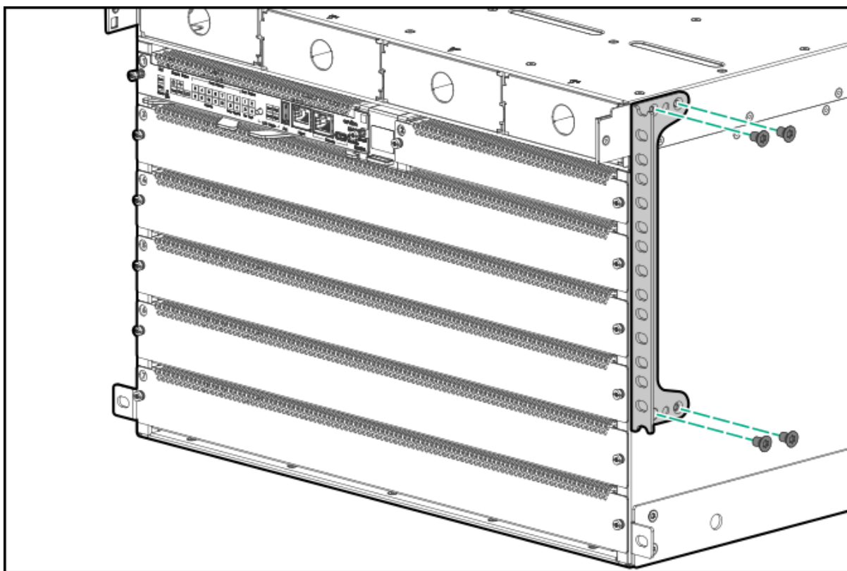
Figure 22 Rack mounting brackets in mounting position 1 on the Aruba 6405 Switch
