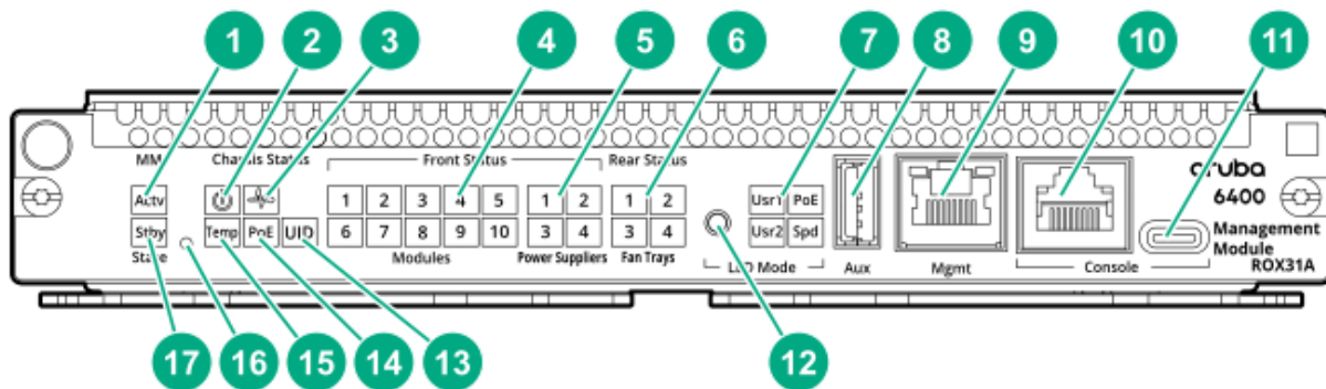
Figure 9 Management module features
