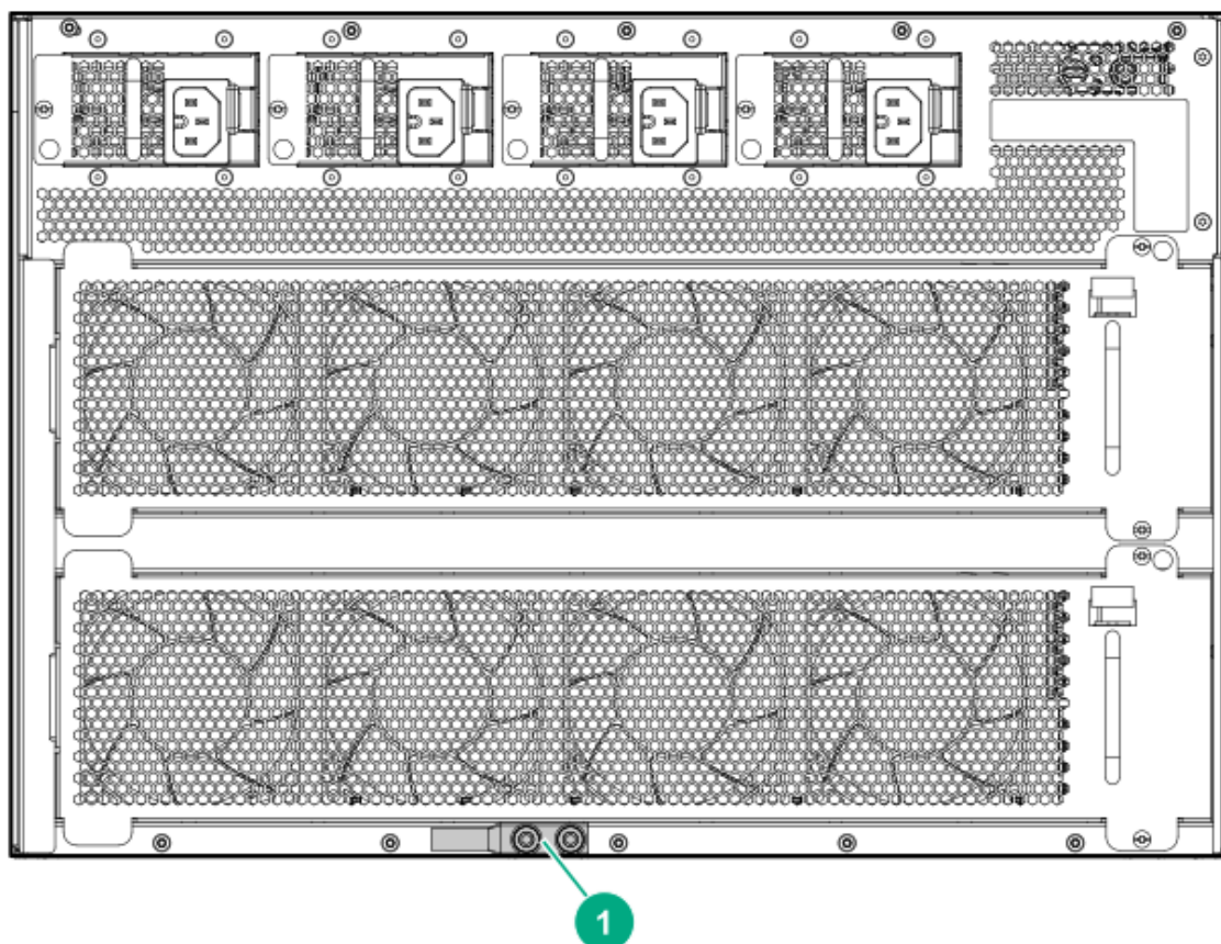
Figure 3 Grounding lug on the HPE Aruba Networking 6405 Switch
