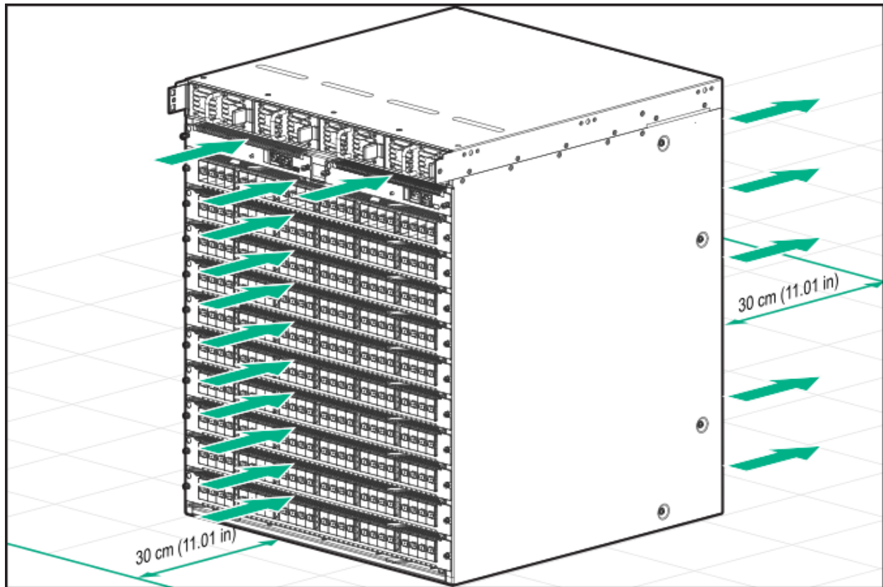
Figure 6 HPE Aruba Networking 6410 Switch Cooling Air Flow
