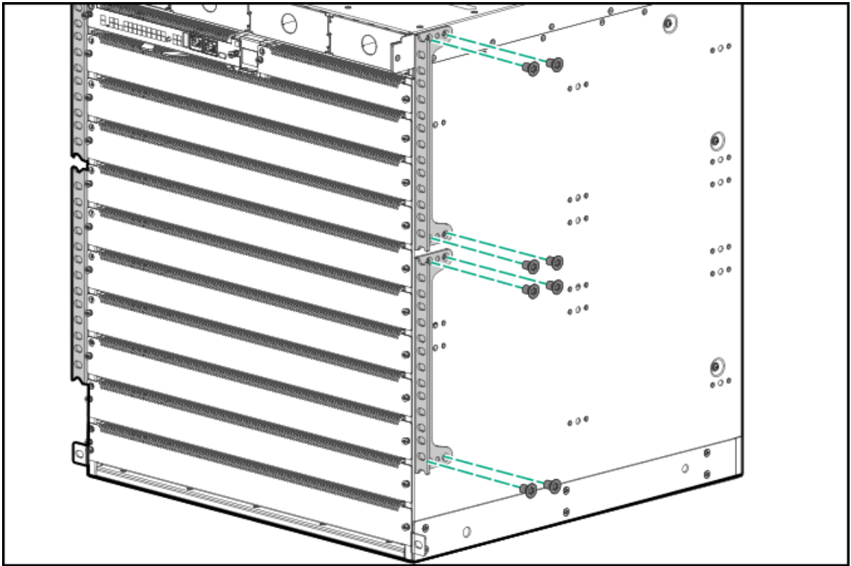
Figure 23 Rack mounting brackets in mounting position 1 on the HPE Aruba Networking 6410 Switch
