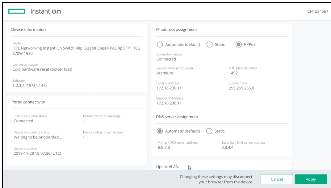
Figure 2 IP Assignment
